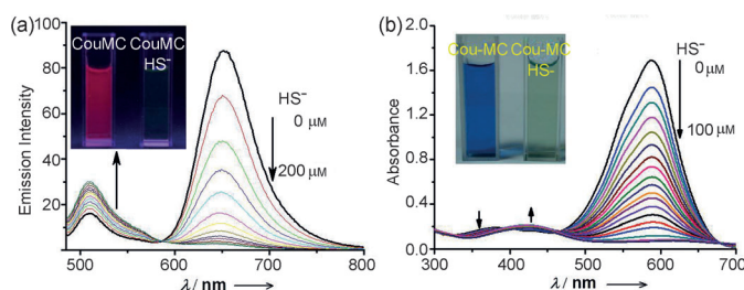
Figure 1. a) Fluorescence spectra of CouMC (10 μM) in PBS (20 mM, pH 7.40, 2% DMSO, v/v) obtained upon titration with HS − from 0 to 200 μM. λ ex , 475 nm. b) Absorption spectra of CouMC (25 μM) in PBS (20 mM, pH 7.40, 5% DMSO, v/v) obtained upon titration with HS − from 0 to 100 μM. Inset in (a): photograph of CouMC solutions upon irradiation by a UV lamp (365 nm) in the absence or presence of HS − . Inset in (b): photograph of CouMC solutions in the absence or presence of HS − .
